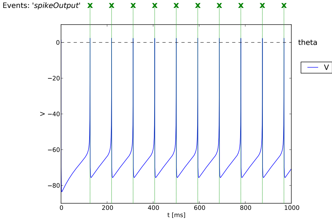
Fig. 6.2: Result of simulating of the XML model in this section
