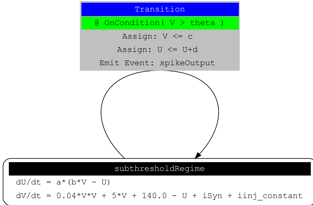
Fig. 6.1: RegimeGraph for the XML model in this section.
